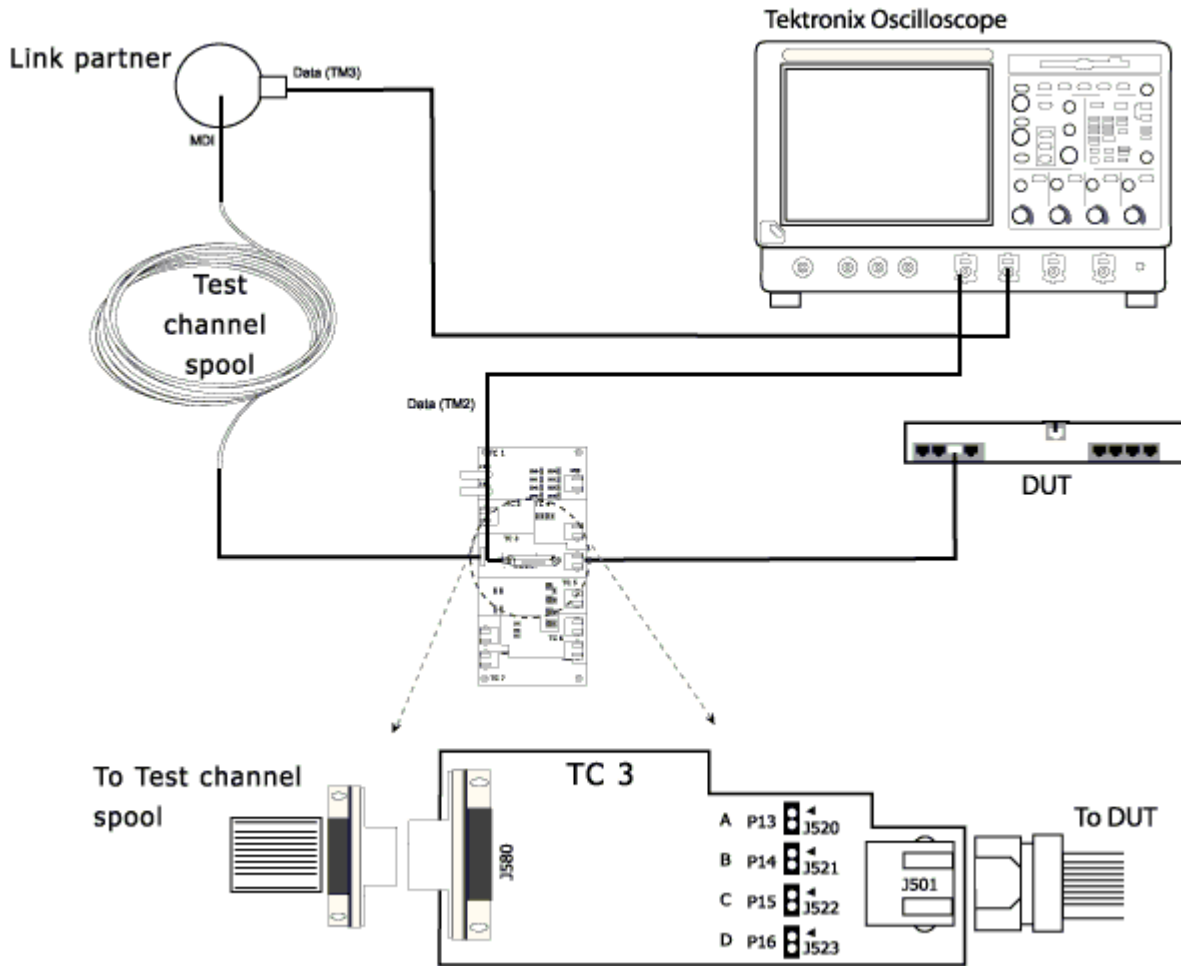
Figure 6-12: 1000BASE-T Connections for Jitter Slave Unfiltered
