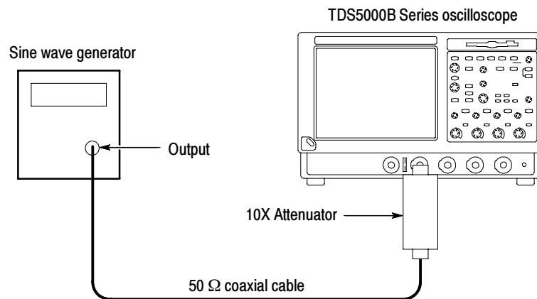
Figure 2- 18: Initial test hookup
