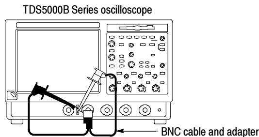
Figure 2- 24: Initial test hookup
