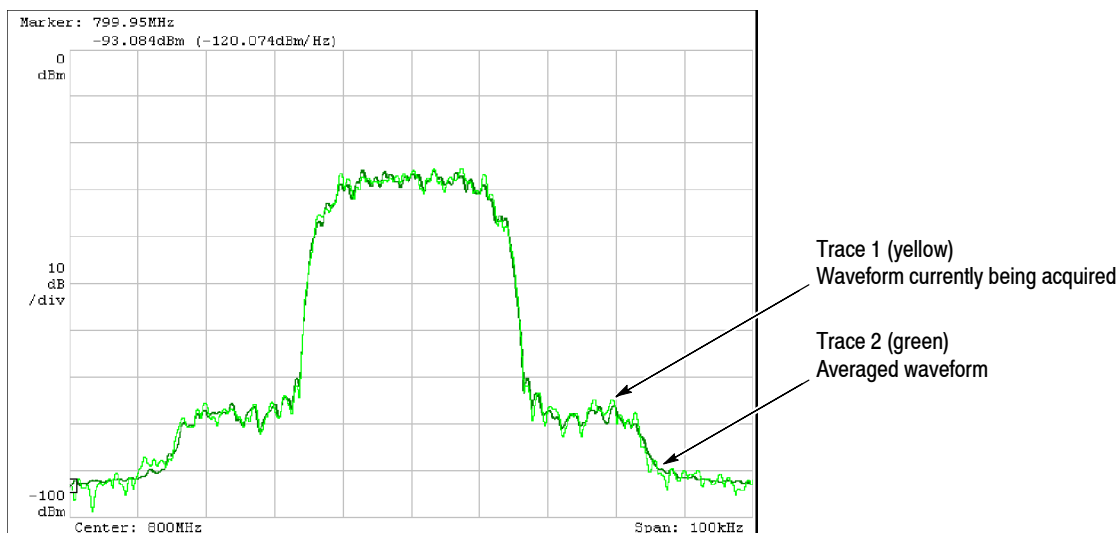
Figure 3-128: Comparison display of Trace 1 and 2
