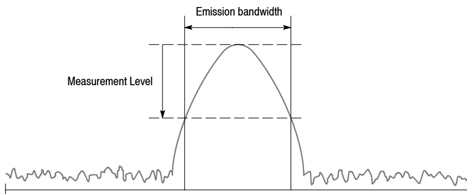
Figure 3- 13: EBW measurement band power markers
