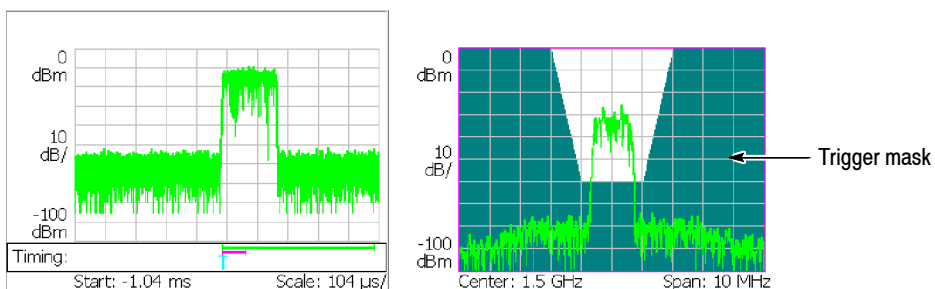
Figure 3-113: Trigger mask
