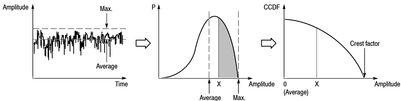
Figure 3-66: CCDF calculation process
