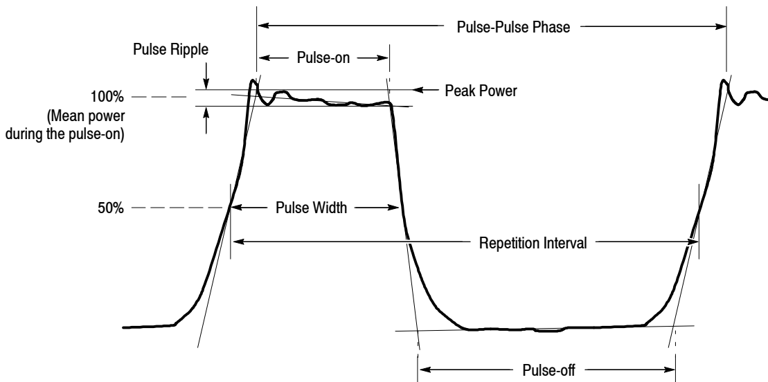
Figure 3-69: Definition of pulse characteristics
