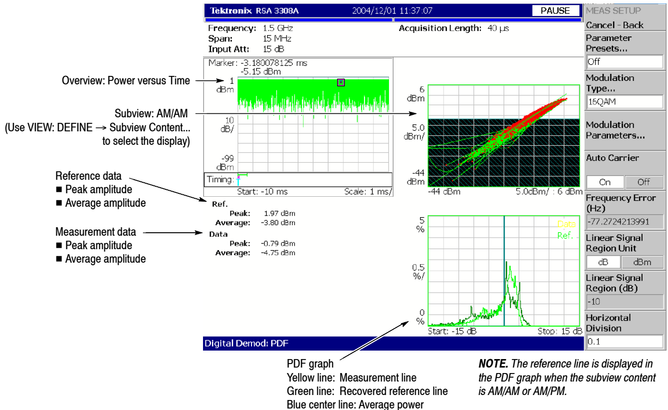
Figure 3-50: PDF measurement
