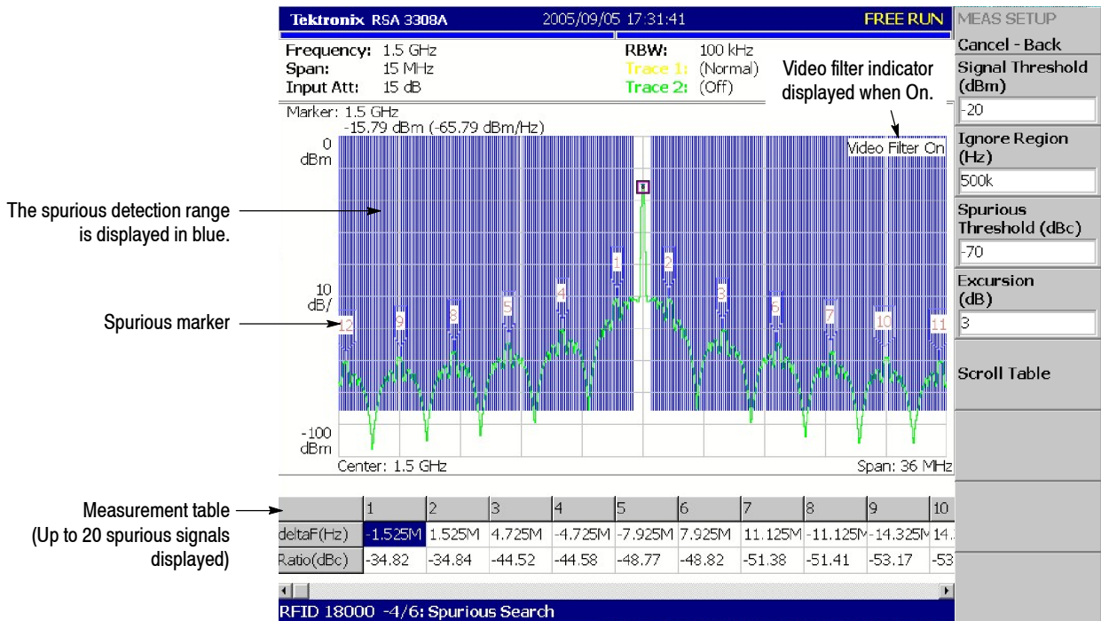
Figure 3-53: Spurious measurement
