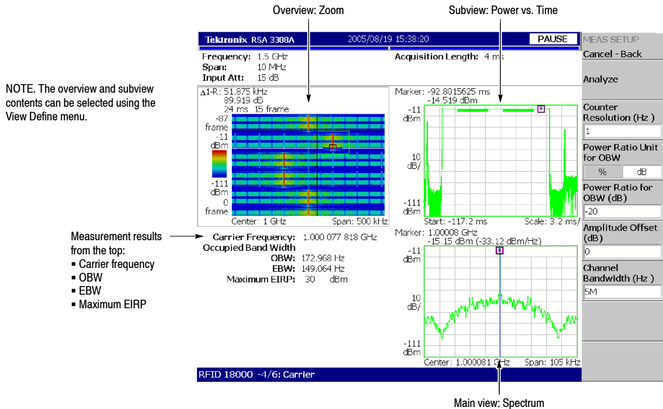
Figure 3- 52: Carrier measurement
