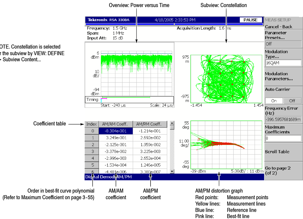
Figure 3-48: AM/PM measurement
