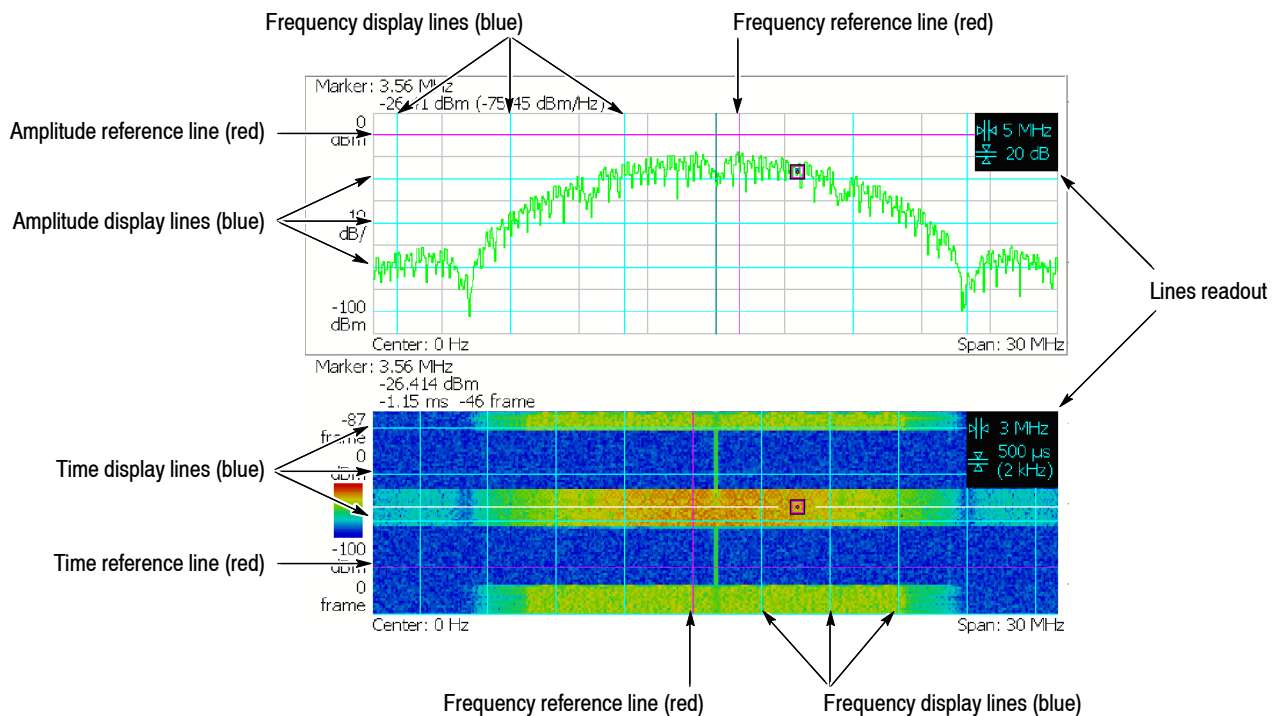
Figure 3-153: Multi display lines (Real Time S/A mode)
