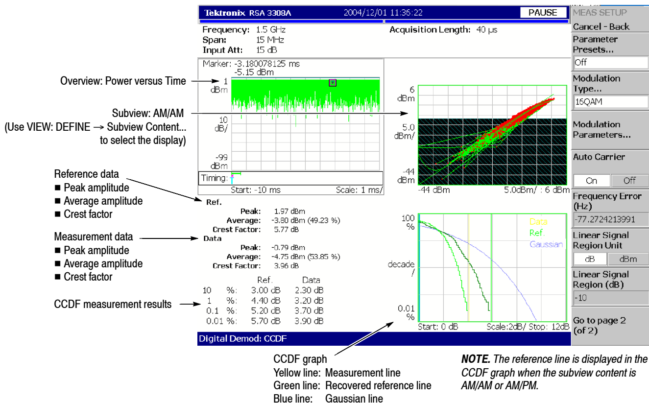
Figure 3-49: CCDF measurement
