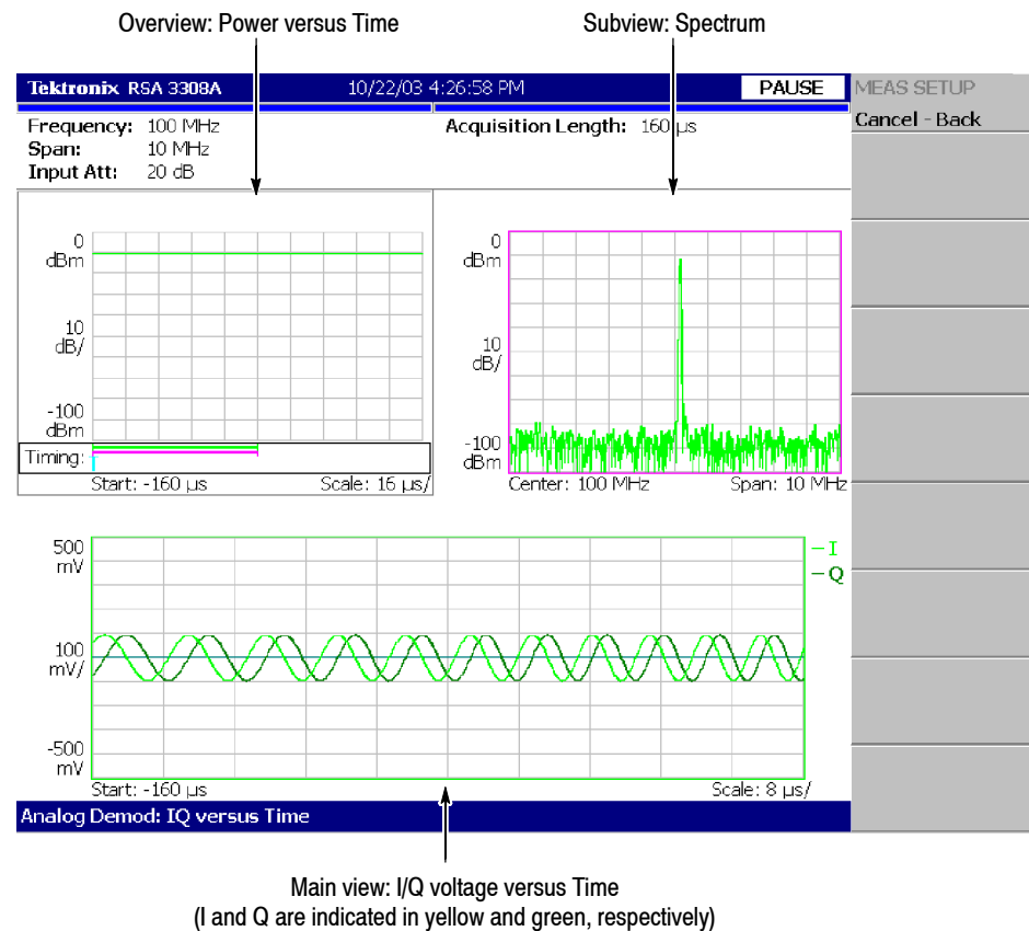
Figure 3-37: IQ versus time measurement
