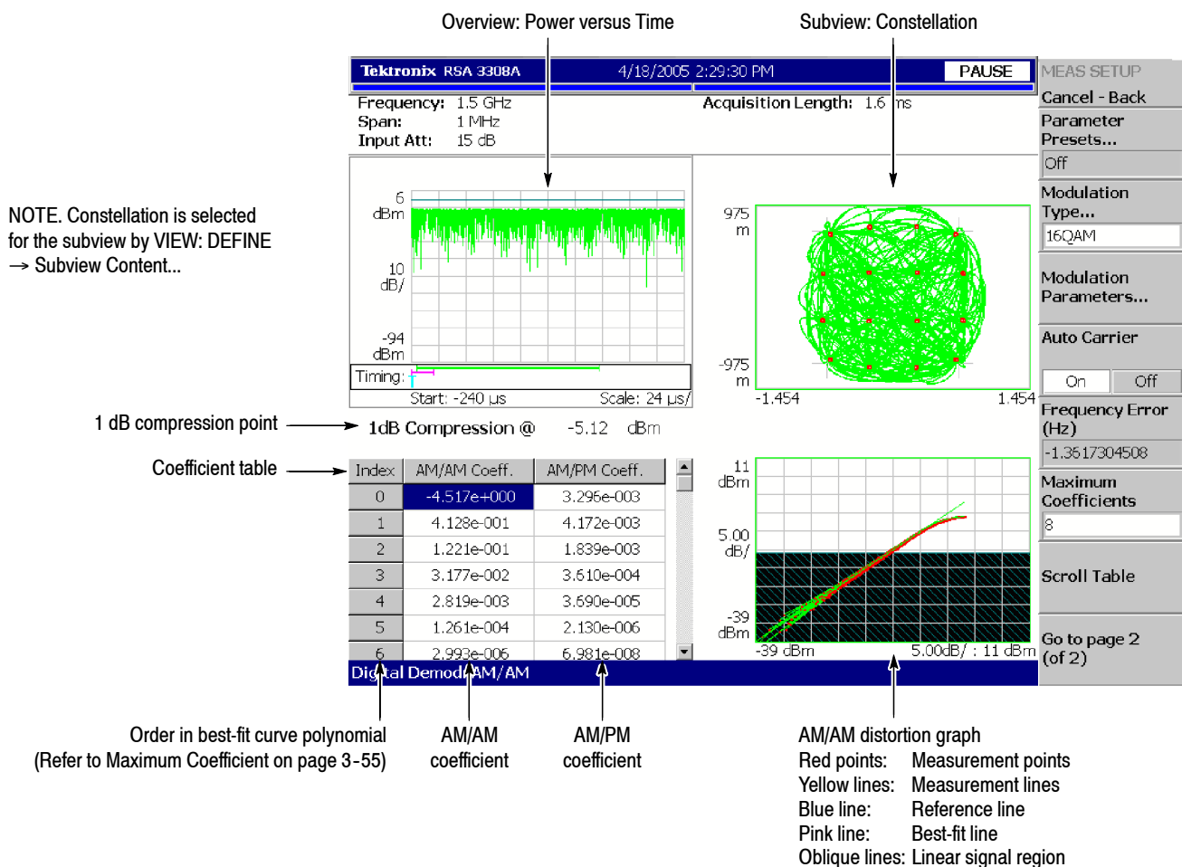
Figure 3-47: AM/AM measurement
