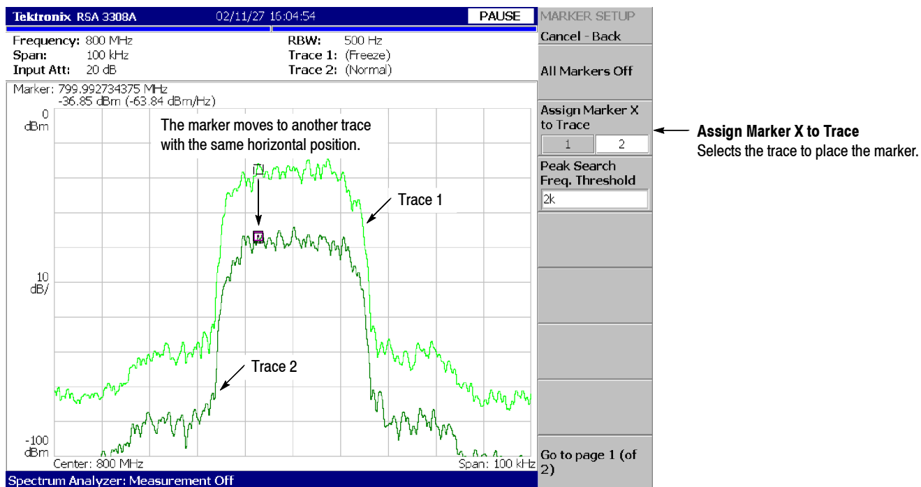
Figure 3- 160: Changing the Trace
