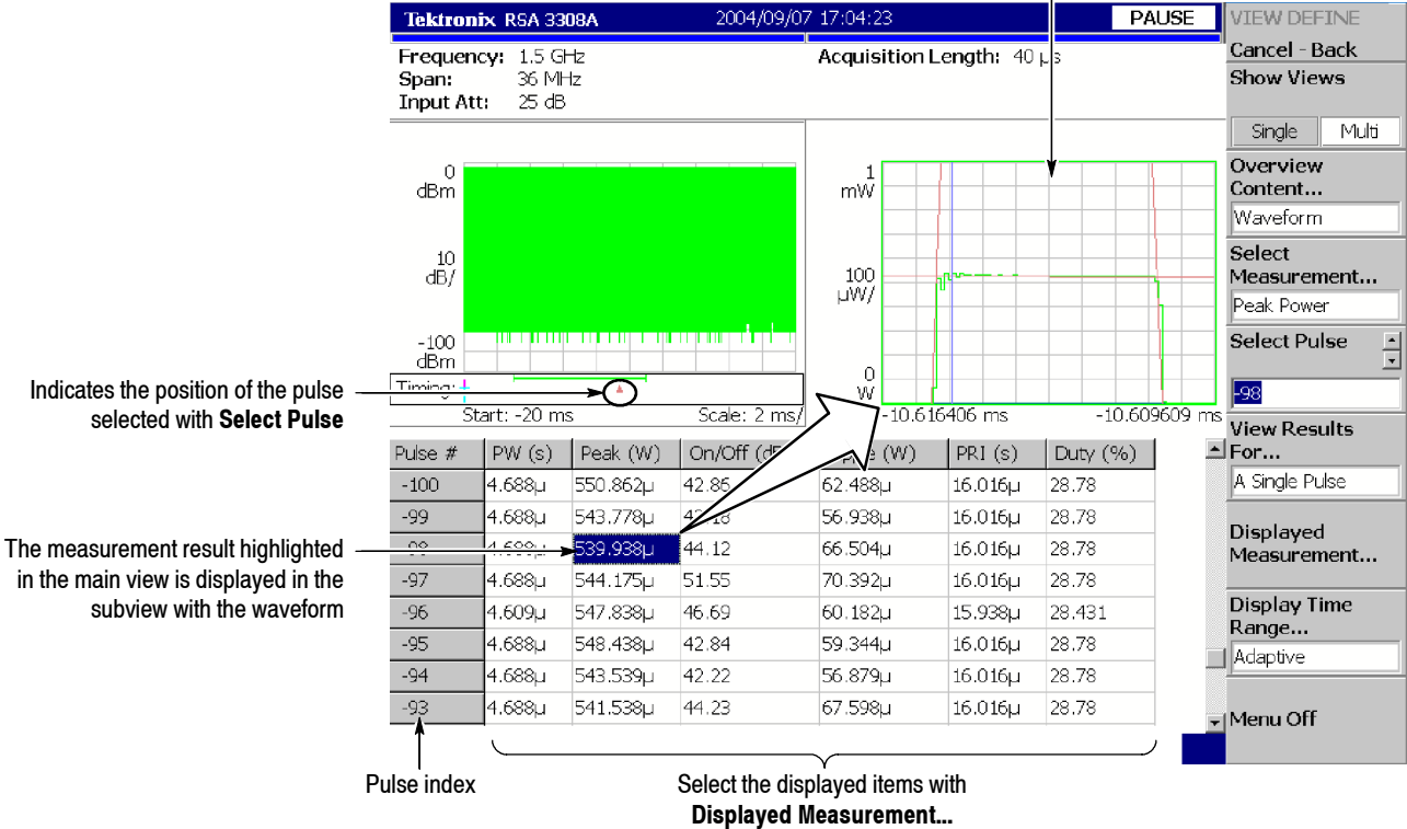
Figure 3-72: Setting the View Define menu
