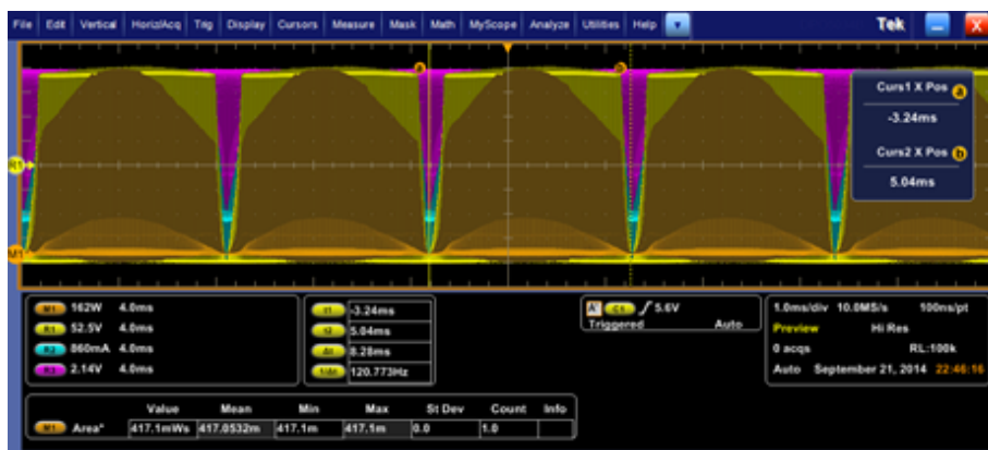
Figure 24: Cursor placement
