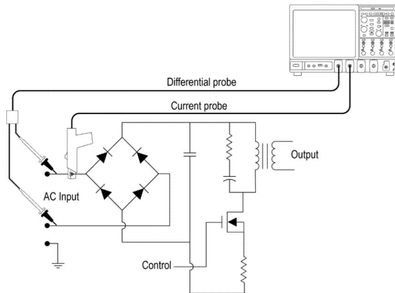
Figure 14: Equipment setup for Pulse Width analysis
