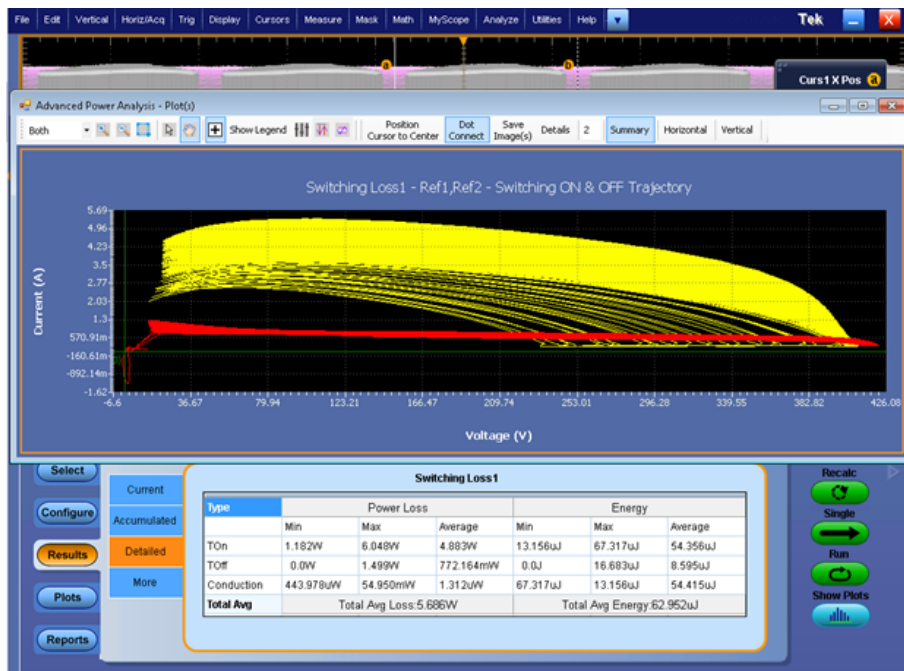
Figure 27: Measurement results and switching loss plot
