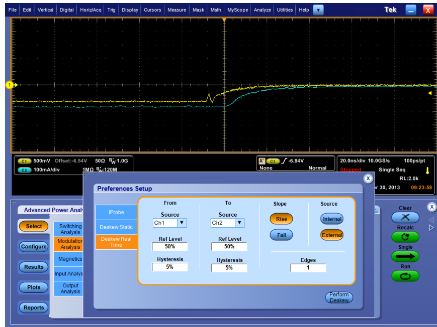
Figure 1: Waveform before deskew
