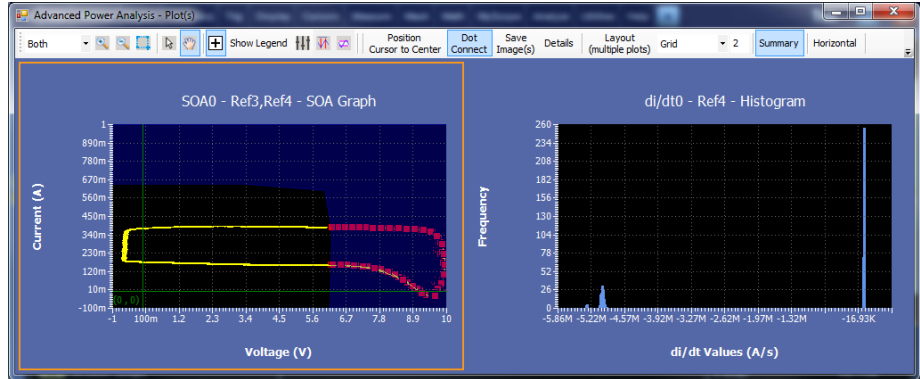
Figure 3: Plot with violation
