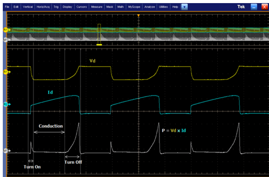
Figure 30: Switching Loss TOn, TOff and Conduction loss regions
