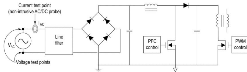
Figure 22: SMPS circuit diagram
