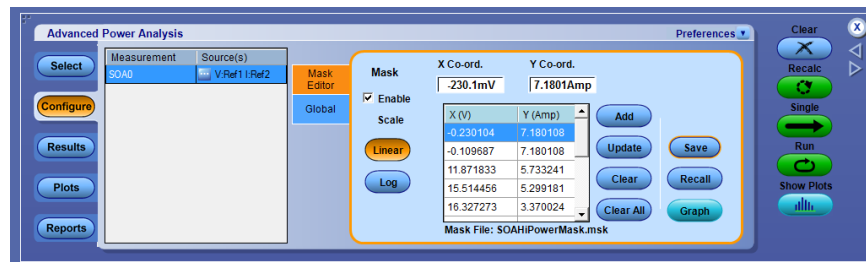
Figure 12: SOA configuration
