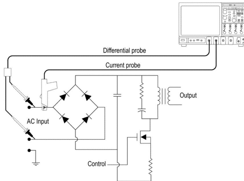
Figure 15: Equipment setup for Pulse Quality analysis
