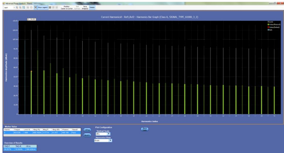
Figure 16: Even harmonics bar graph
