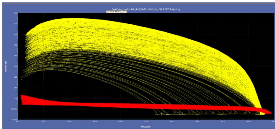
Figure 44: Typical PFC plot over many cycles
