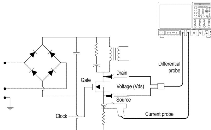
Figure 19: Equipment connection setup for Hi-Power finder
