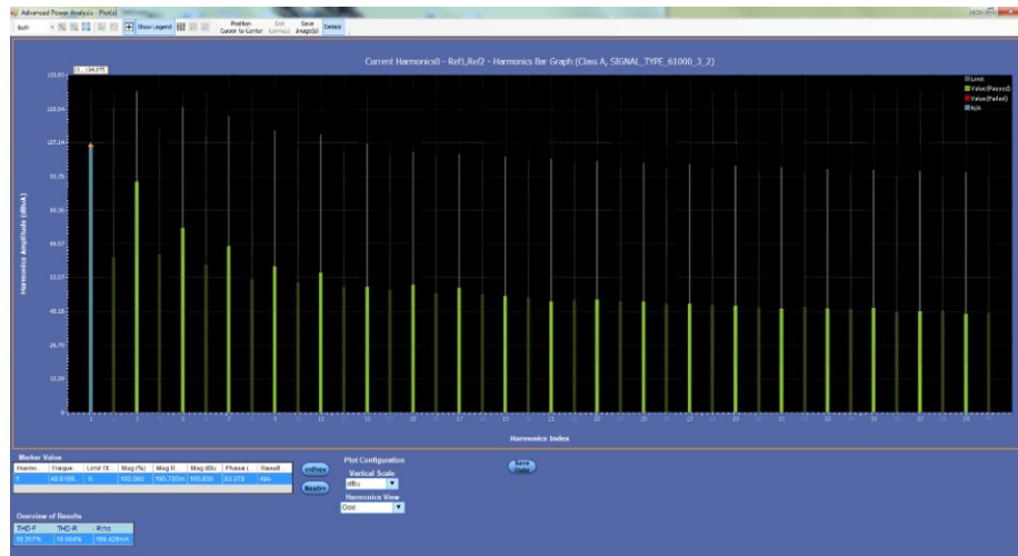
Figure 17: Odd harmonics bar graph
