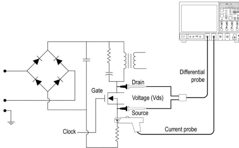
Figure 11: Equipment setup for Safe Operating Area
