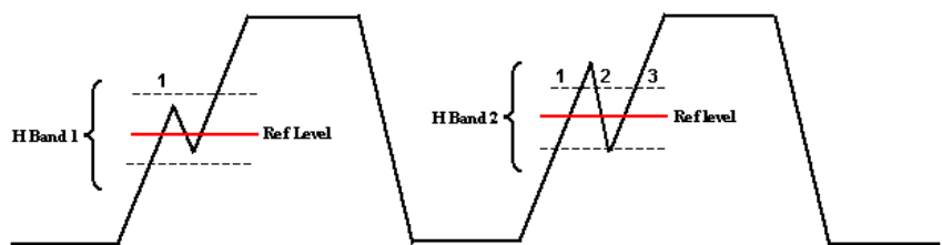
Figure 28: Hysteresis
