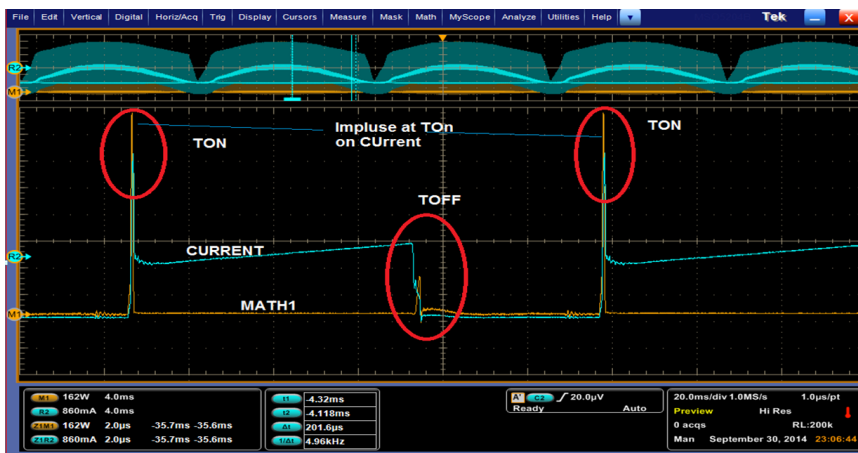
Figure 34: Impulsive current signal
