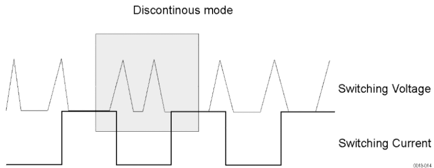
Figure 32: Discontinuous switching mode
