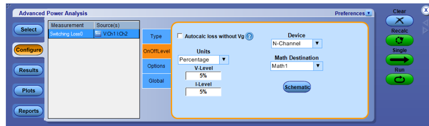
Figure 36: Switching Loss On and OnOff Level configuration
