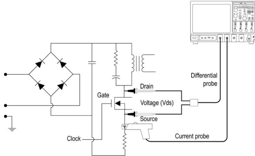
Figure 18: Equipment connection setup for Switching loss
