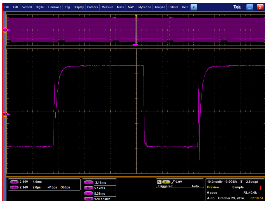
Figure 25: Ringing VG during TOFF
