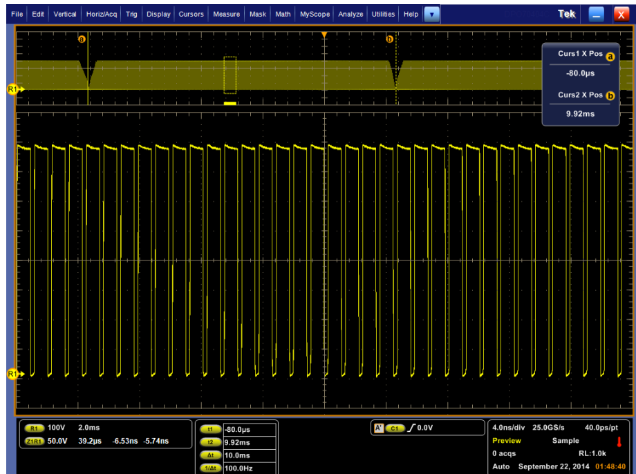
Figure 39: Zoom-in of the VDS (Drain-Source) Voltage Switching cycles
