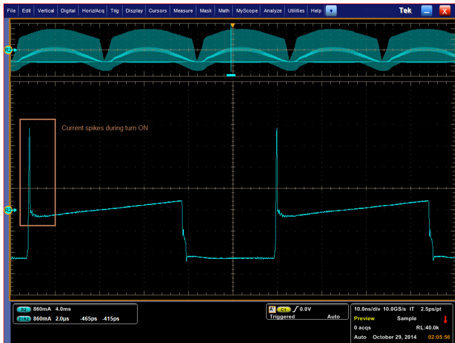
Figure 23: Current spikes during turn ON
