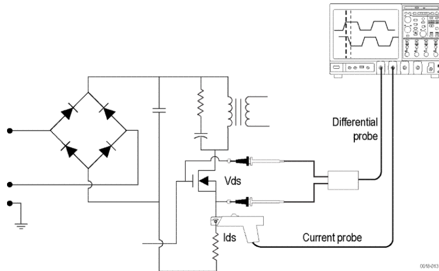
Figure 29: SMPS circuit diagram
