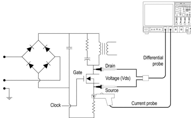
Figure 20: Equipment connection setup for Magnetic loss
