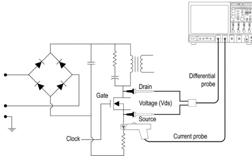
Figure 13: Equipment setup for Safe Operating Area X-Y
