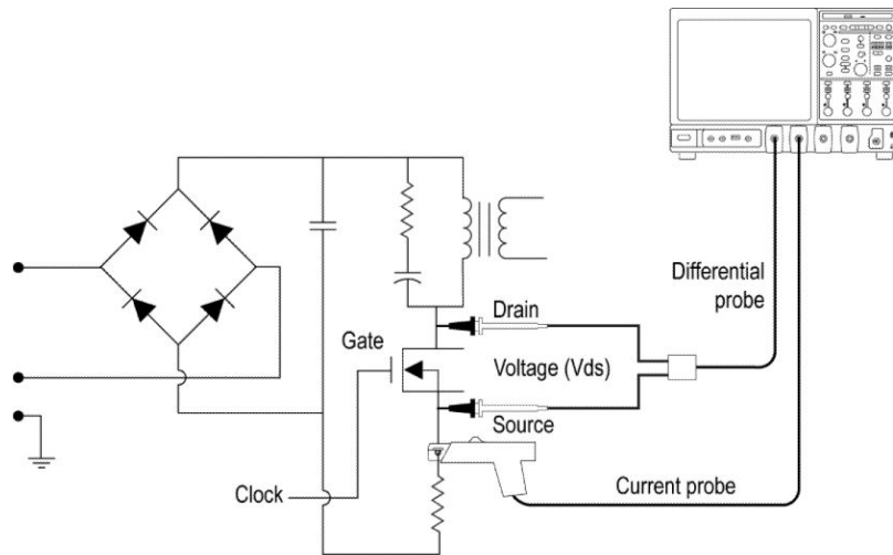
Figure 10: Equipment setup for RDS(on)
