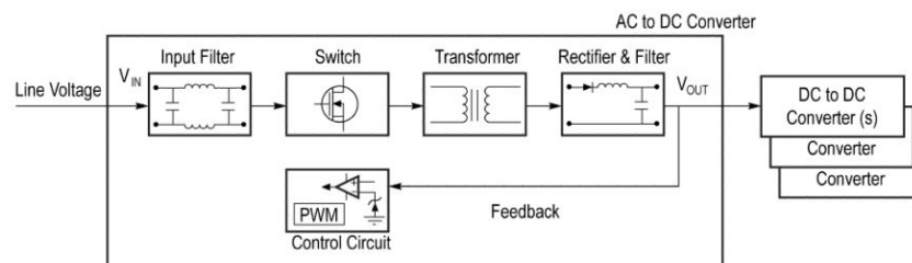
Figure 21: SMPS block diagram
