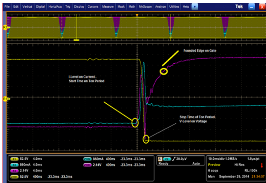
Figure 37: Spike on V_g source
