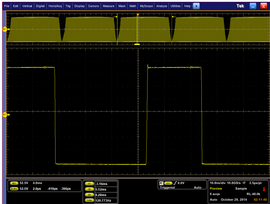
Figure 26: Clean VDS
