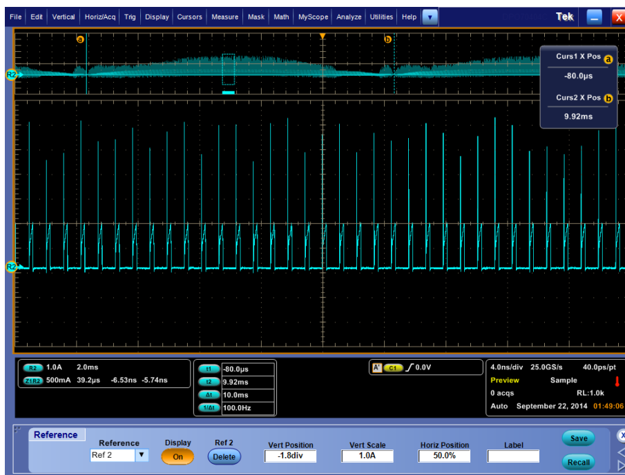
Figure 40: Zoom-in of the IDS (Drain-Source) Current Switching cycles
