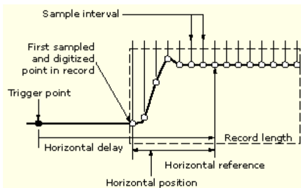
Figure 18: The waveform record and its defining parameters (horizontal delay on)
