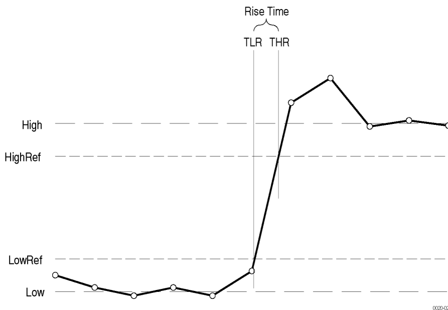
Figure 21: Rise Time
