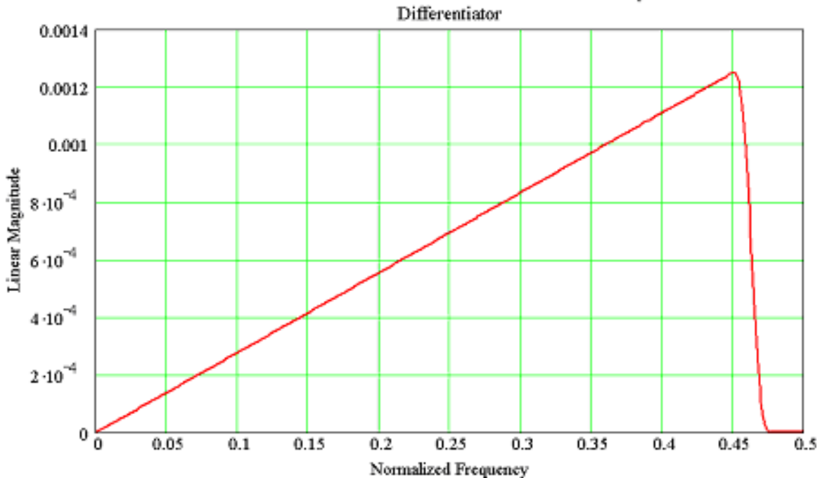
Figure 28: Frequency response of the differentiator filter
