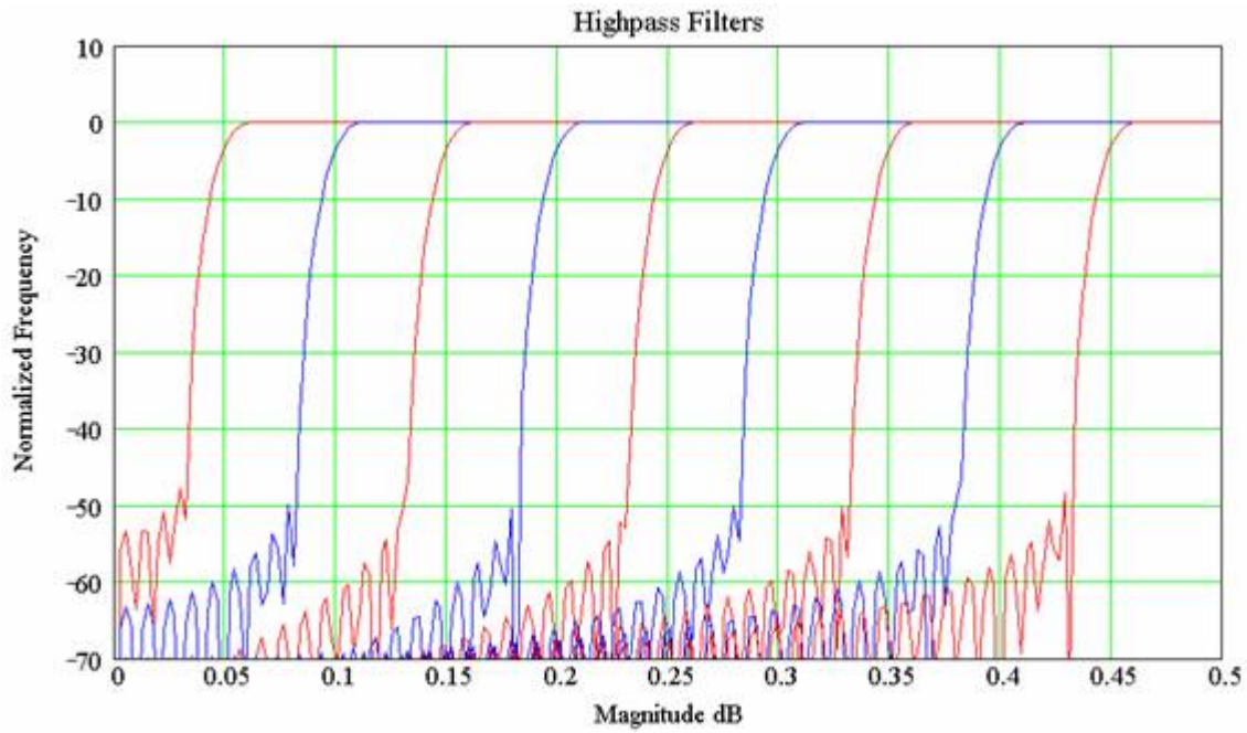
Figure 24: Frequency response of the available high pass filters
