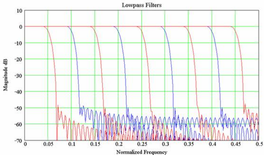
Figure 23: Frequency response of the available low pass filters
