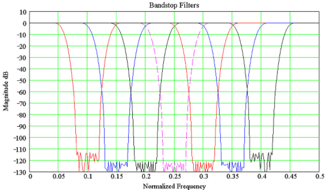
Figure 25: Frequency response of the available band stop filters
