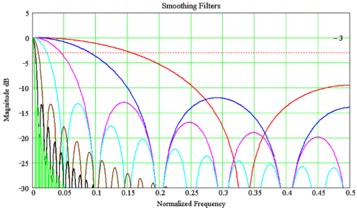
Figure 26: Frequency response of the available smoothing filters
