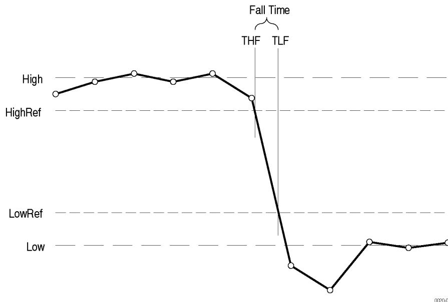
Figure 20: Fall Time
