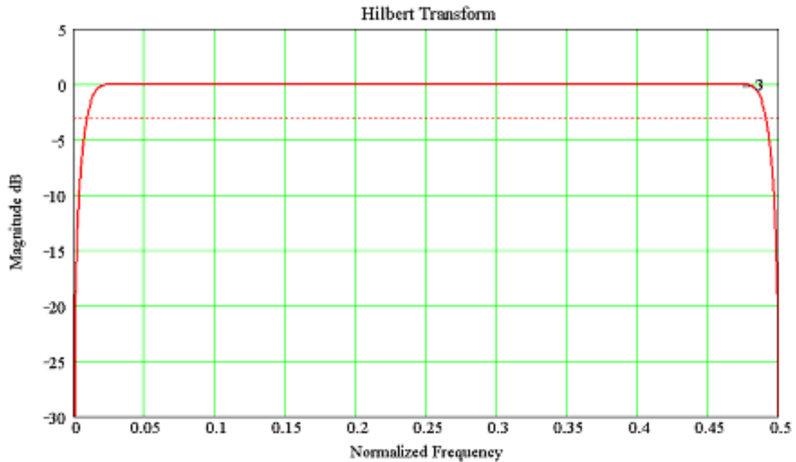
Figure 27: Frequency response of the Hilbert transform filter
