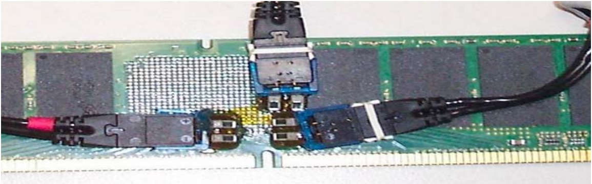
Figure 5: NEX-TDSFBDP test fixture
