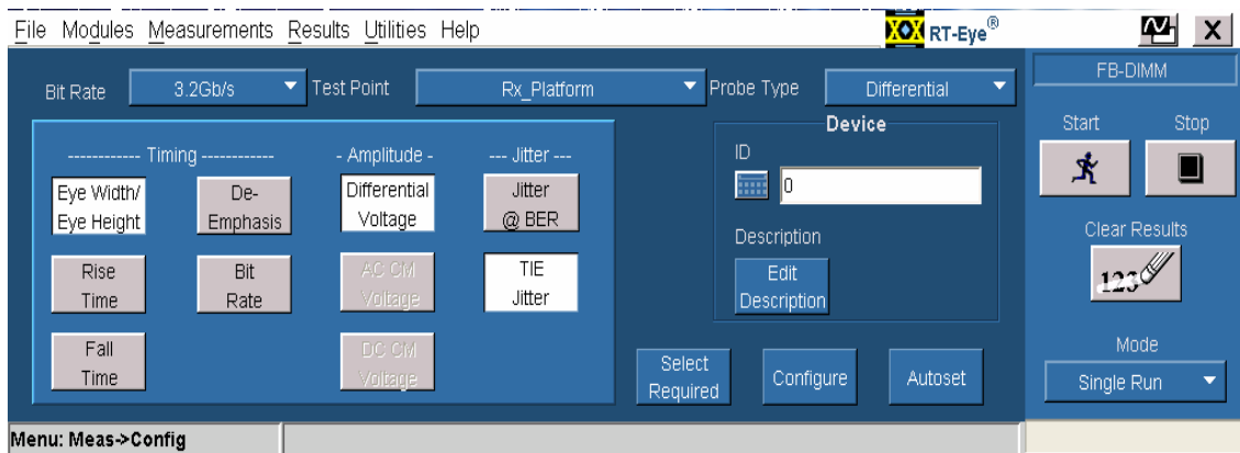
Figure 6b: Measurements select menu setup for Receiver Platform test point with SSC off when tested using the TDSN4238B/Intel's DLB fixture
