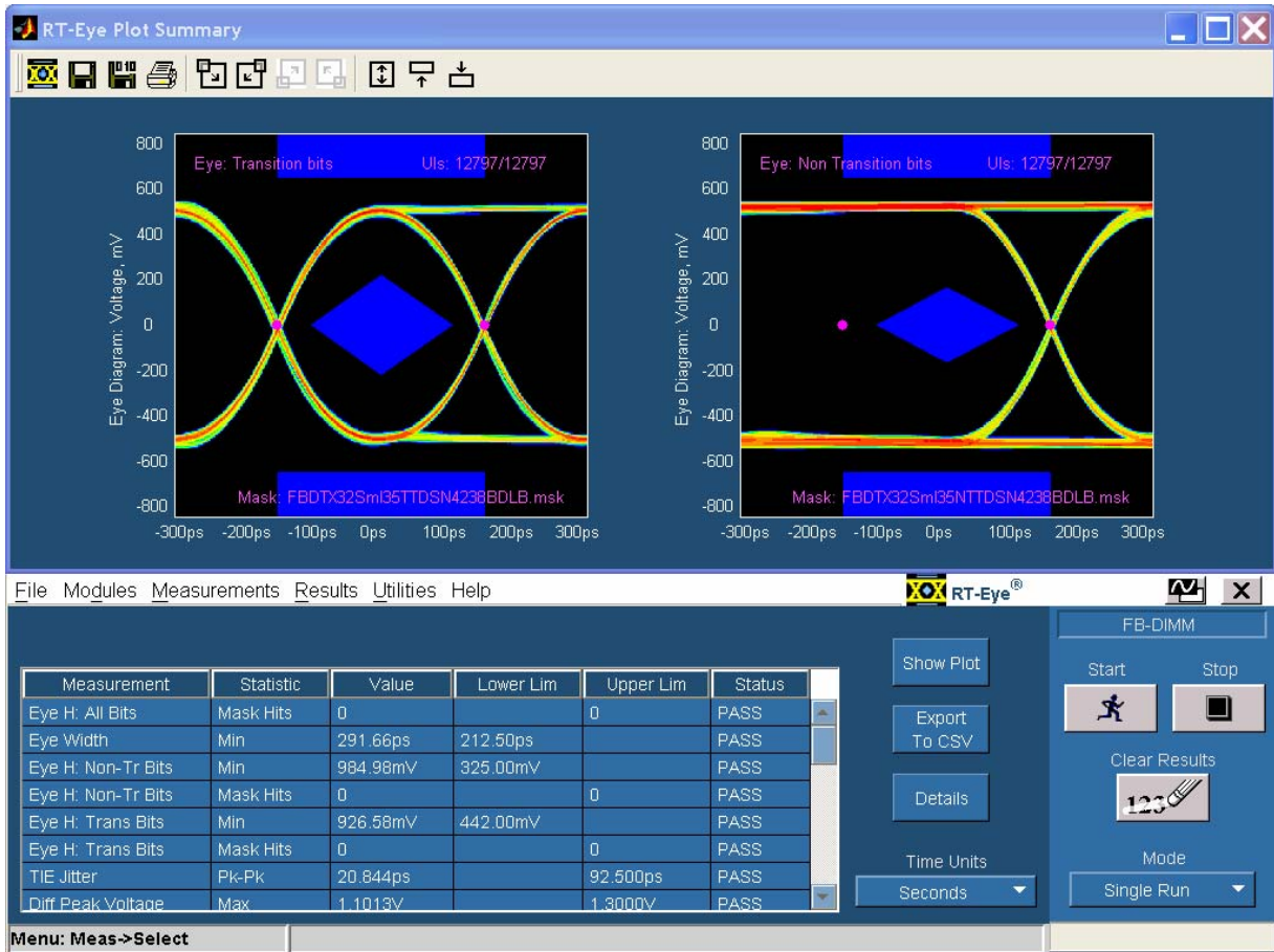
Figure 10b: Result of a completed compliance test on selecting transmitter DIMM test point while using the TDSN4238B/Intel DLB fixture
