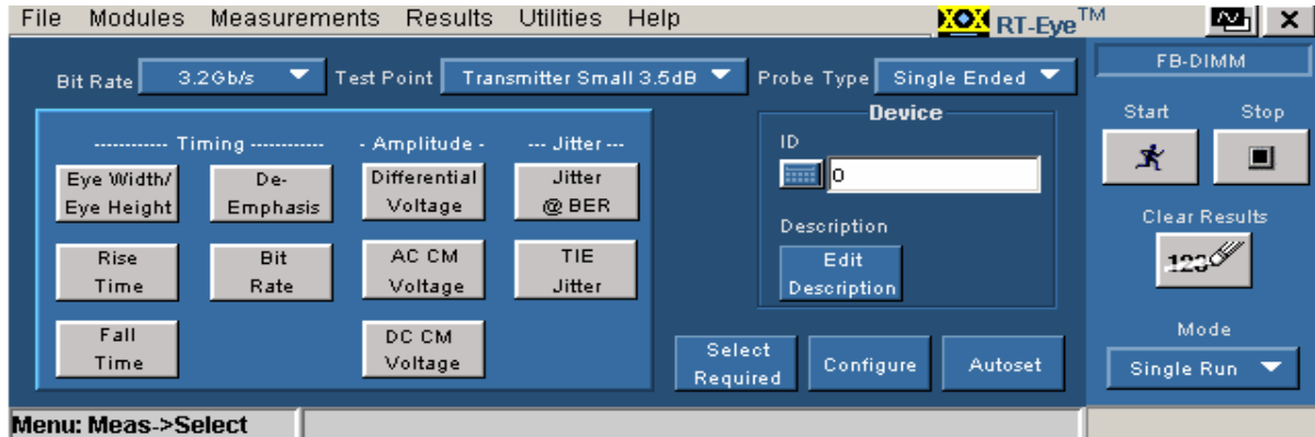
Figure 9a: Measurements select menu setup for Transmitter small/regular/large 3.5db or 6dB de-emphasis levels as per FBDIMM specifications
