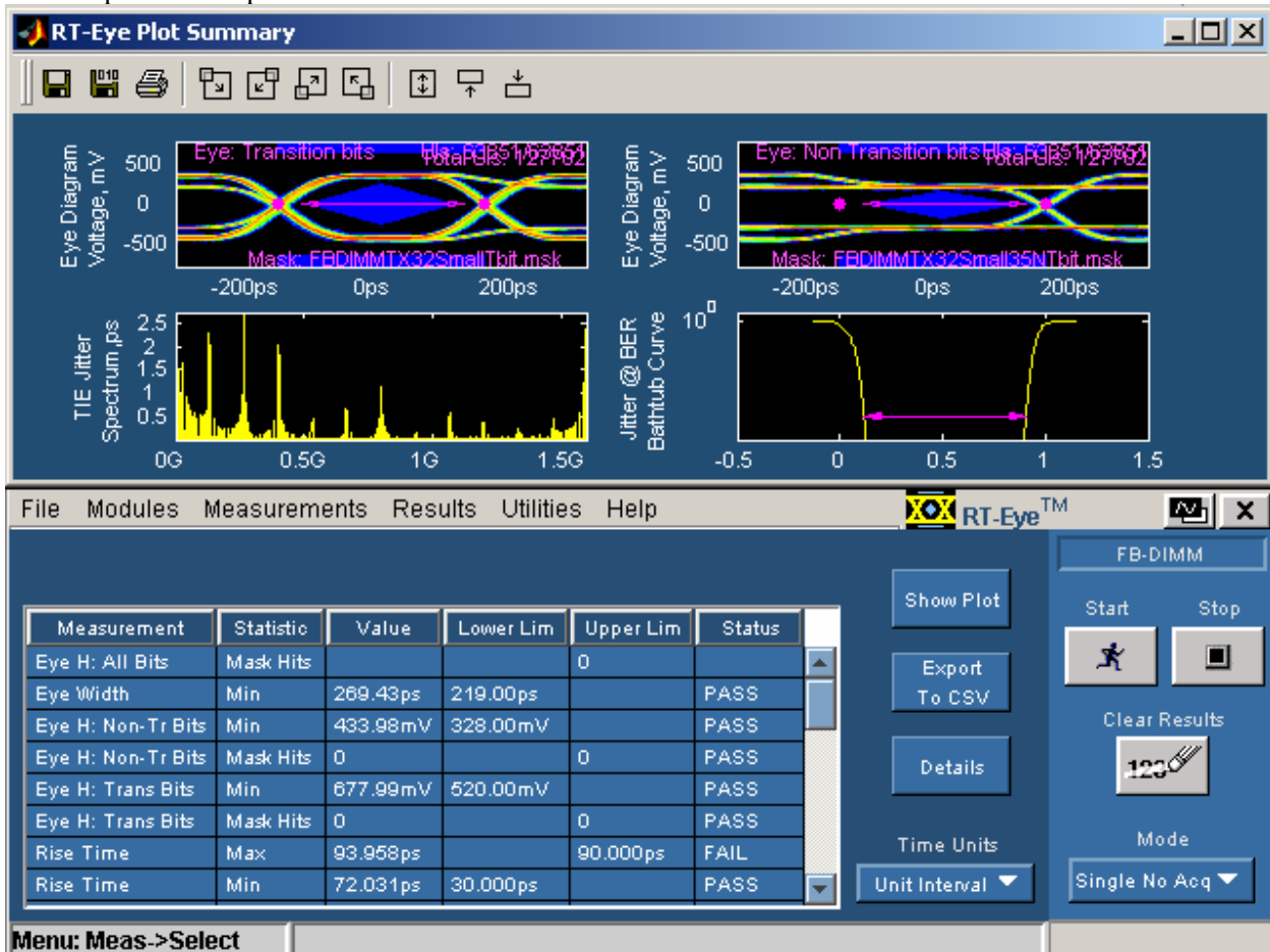
Figure 10a: Result of a completed compliance test at the transmitter pins as per FB-DIMM specifications
