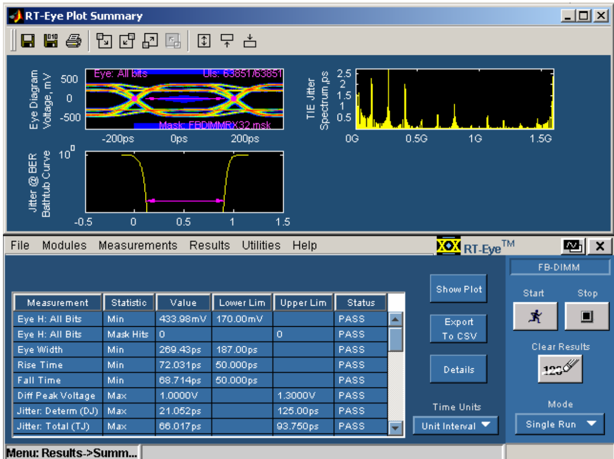
Figure 7a: Result of completed receiver compliance test as per FB-DIMM spec
