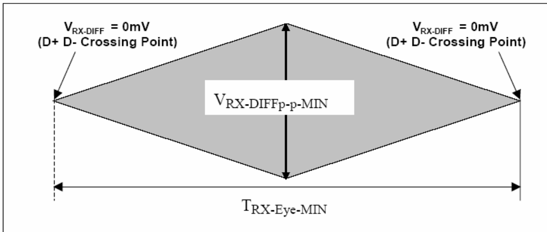
Figure 2: Receiver input eye voltage and timing specifications
