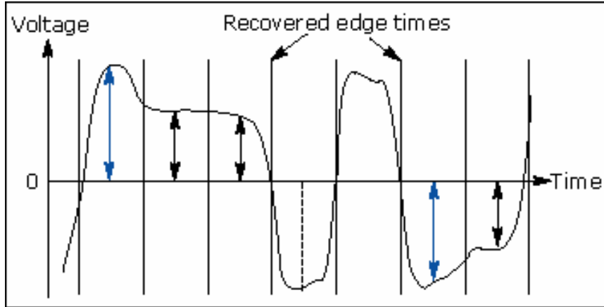
Figure 11: De-emphasis measurement
