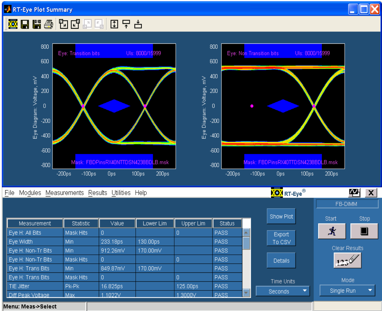
Figure 7b: Result of completed receiver platform compliance test (SSC On/Off) when tested using TDSN4238B/Intel's DLB fixture
