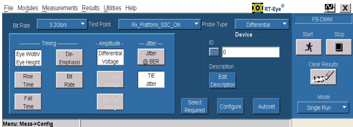
Figure 6c: Measurements select menu setup for Receiver Platform test point with SSC on when tested using the TDSN4238B/Intel's DLB fixture
