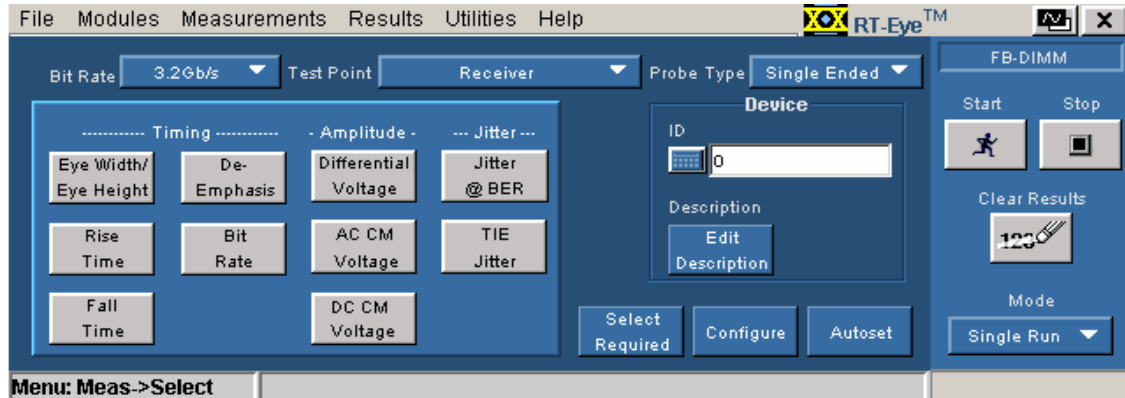
Figure 6a: Measurements select menu setup for Receiver test point as per FBDIMM spec
