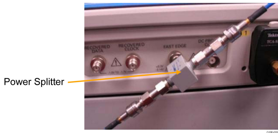
Figure 14: Cable deskew connections
